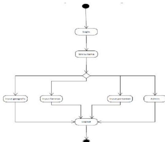
Gambar 3. State Diagram
