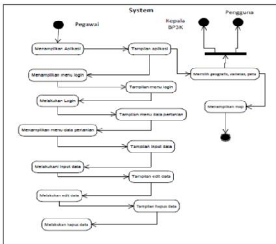
Gambar 2. Activity Diagram
