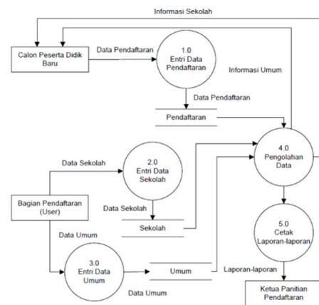
Gambar 2. DFD Level 0
