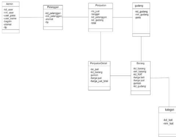
Gambar 2.4 Class Diagram
