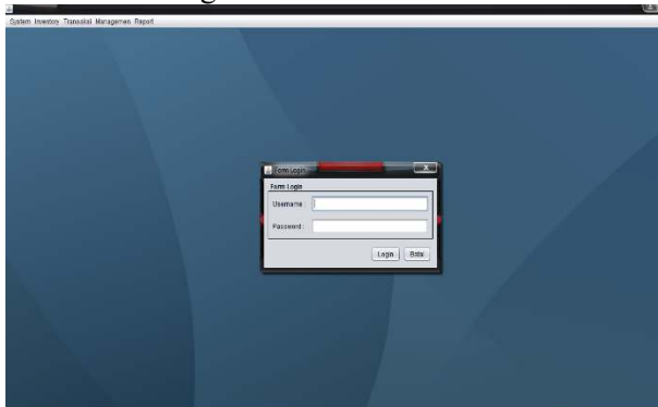
Gambar 3. 2 Form Login
